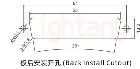
板后安装开孔 (Back Install Cutout)
